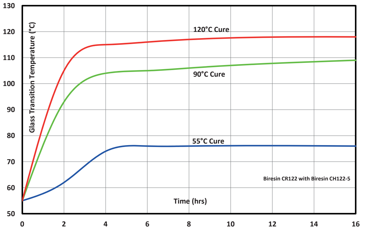
Glass Transition Temperature vs. Cure Cycle, Biresin® CR122 with Biresin® CH122-5
